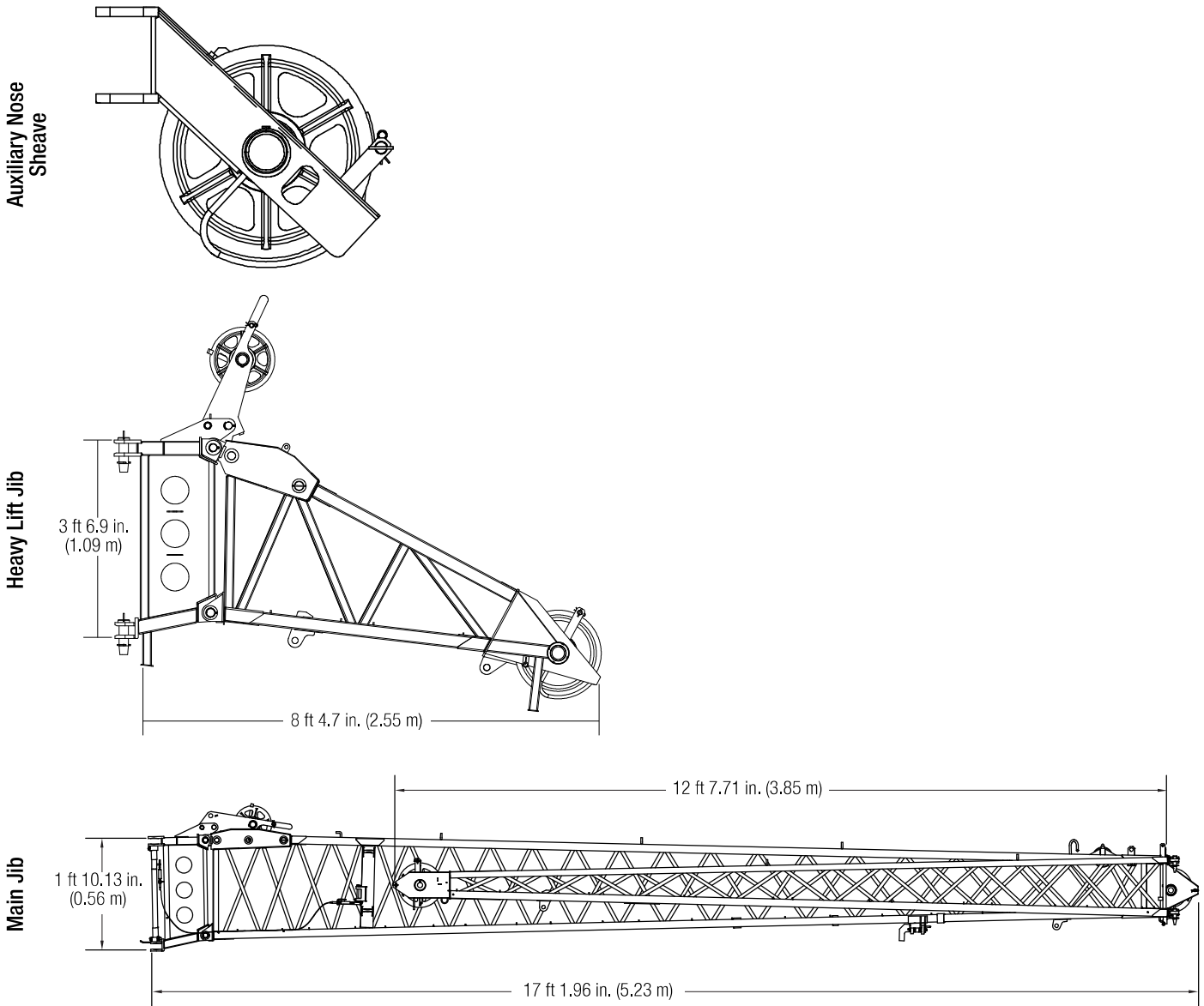
Figure 52: Optional jibs
